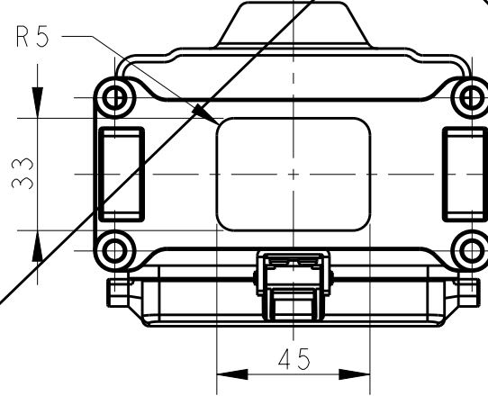
HOUSING 下壳
