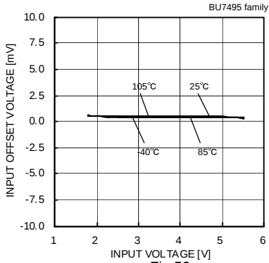
Fig.59 Input Offset Voltage – Supply Voltage (V icm =V DD -1.2[V], V OUT =1.5[V])
