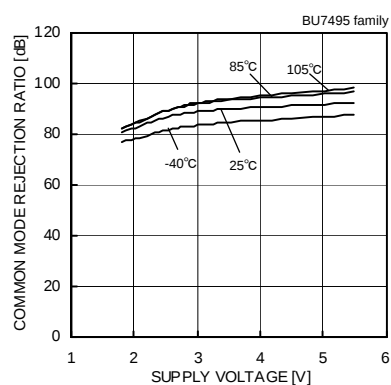
Fig.64 Common Mode Rejection Ratio – Supply Voltage (V DD =3[V])
