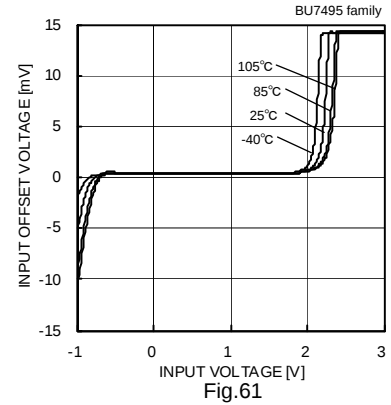
Fig.61 Input Offset Voltage – Input Voltage (V DD =3[V])
