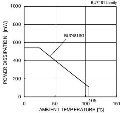
Fig.71 Derating curve
