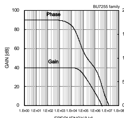
Fig.46 Voltage Gain – Frequency
