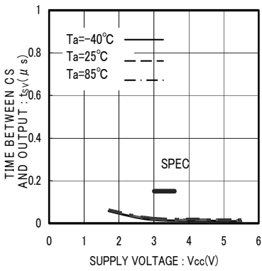
Fig.20 Time from CS to output establishment t sv
