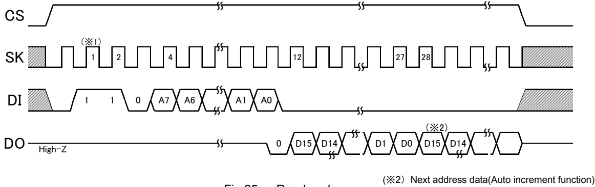
Fig.25 Read cycle
