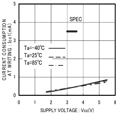
Fig.8 Current consumption at WRITE action Icc1(fsk=2MHz)
