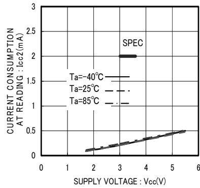
Fig.9 Consumption current at READ action Icc2(fsk=2MHz)
