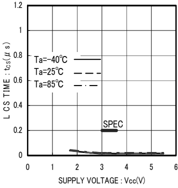
Fig.14 CS Low time t_{cs}
