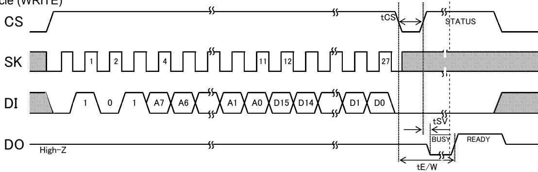
Fig.26 Write cycle
