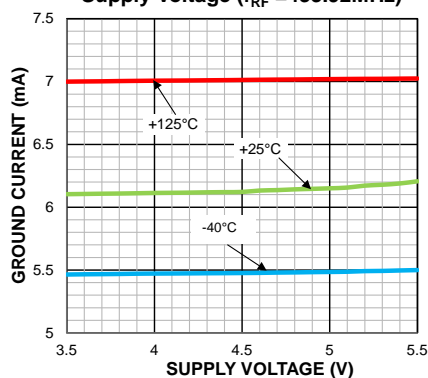
Ground Current vs. Supply Voltage ( f_{RF} = 433.92\text{ MHz} )
