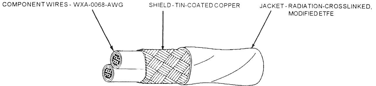
EXAMPLE: CXA-0066-24-2 (TWO CONDUCTOR CABLE)
