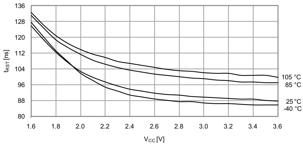
Figure 33-400. Minimum Reset Pin Pulse Width vs. V CC
