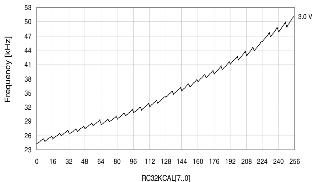
Figure 33-407. 32.768kHz Internal Oscillator Frequency vs. Calibration Value
