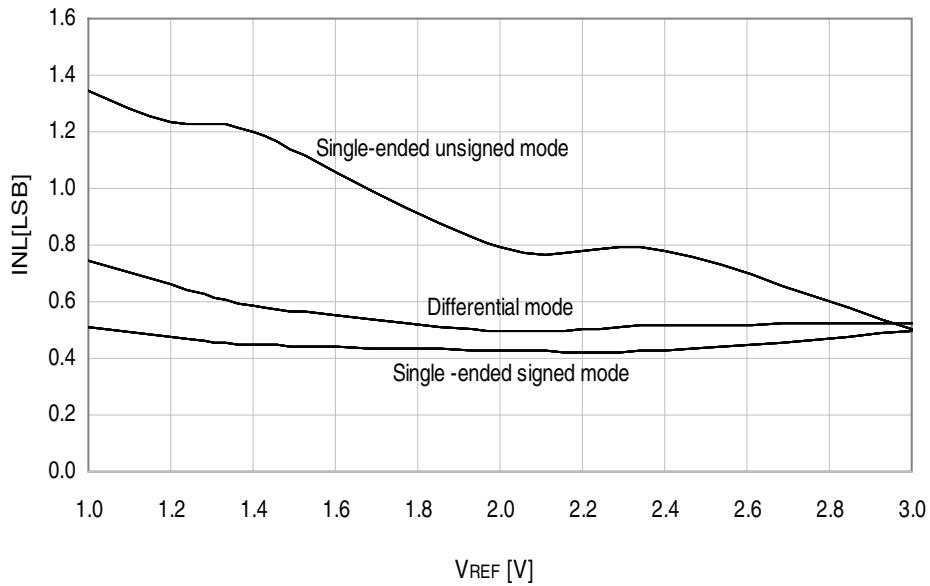
Figure 33-382. INL Error vs. External V_{REF}
