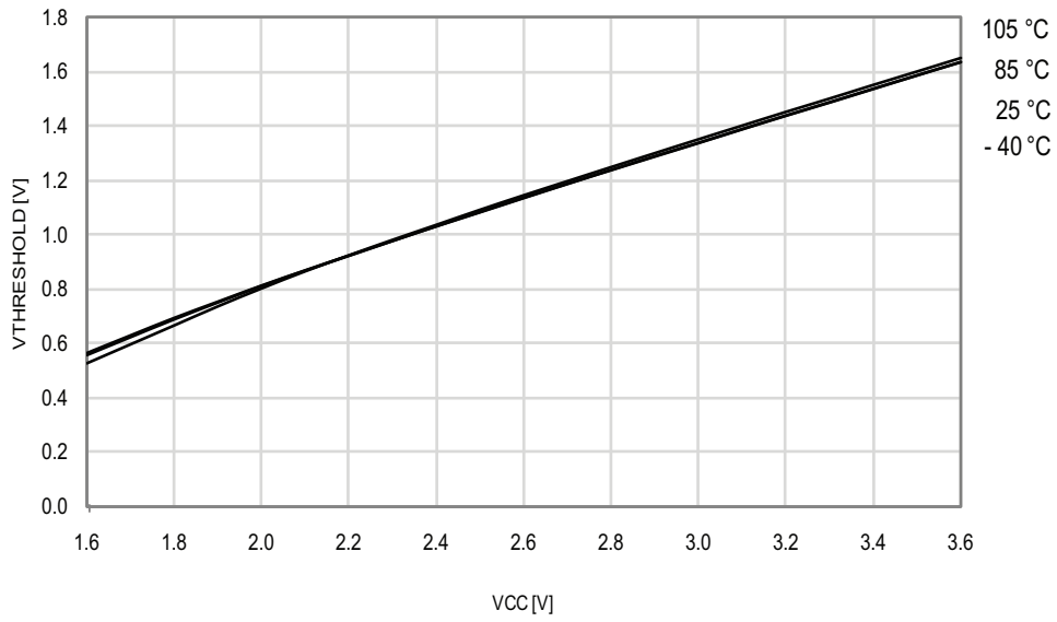
Figure 33-124. Reset Pin Input Threshold Voltage vs. V CC
