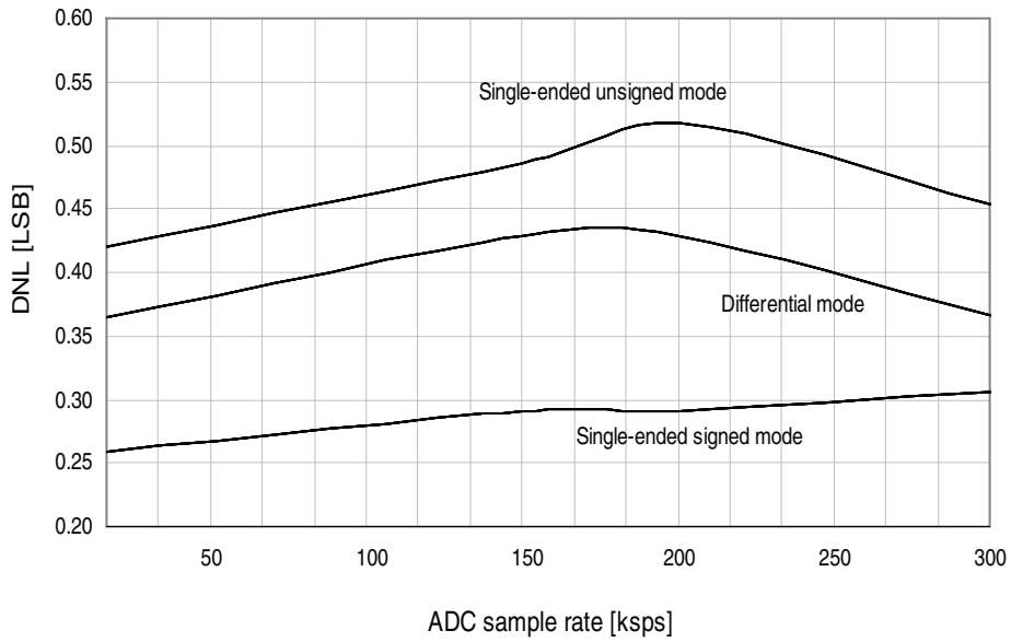
Figure 33-106. DNL Error vs. Sample Rate
