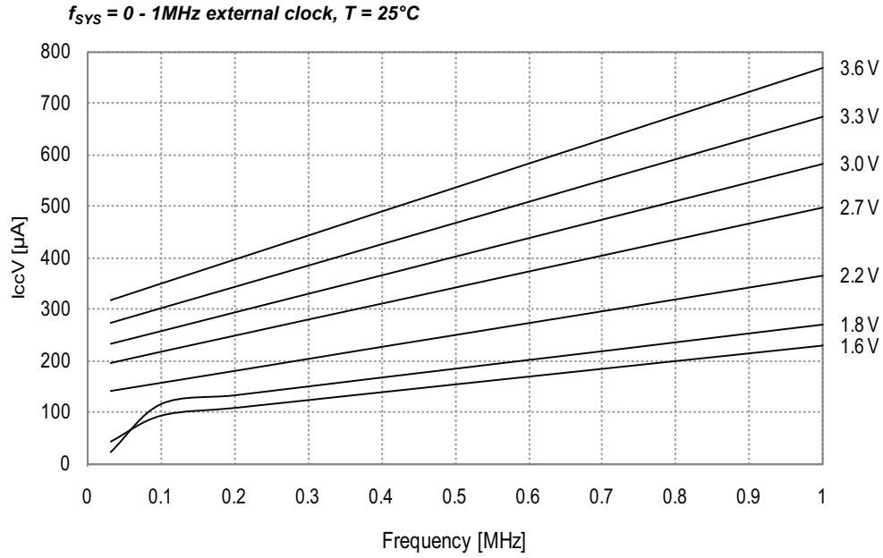
Figure 33-72. Active Supply Current vs. Frequency
