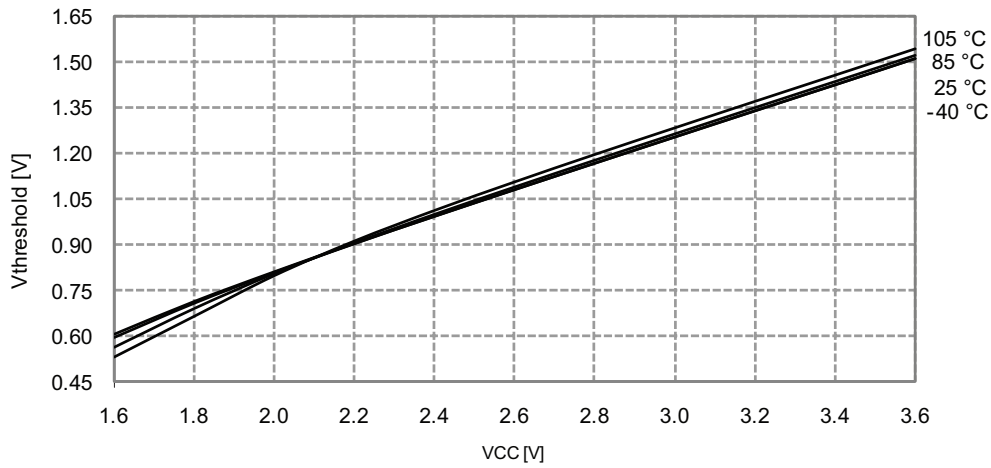
Figure 33-310. I/O Pin Input Threshold Voltage vs. V_{CC}
