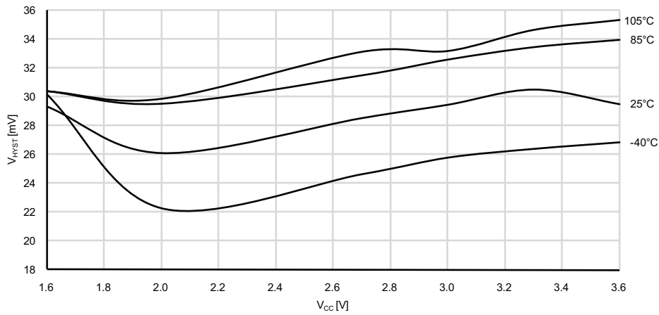
Figure 33-324. Analog Comparator Hysteresis vs. V_{CC} Large hysteresis
