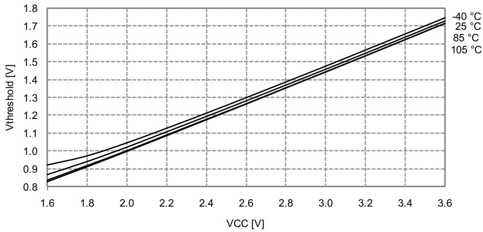
Figure 33-310. I/O Pin Input Threshold Voltage vs. V_{CC}
