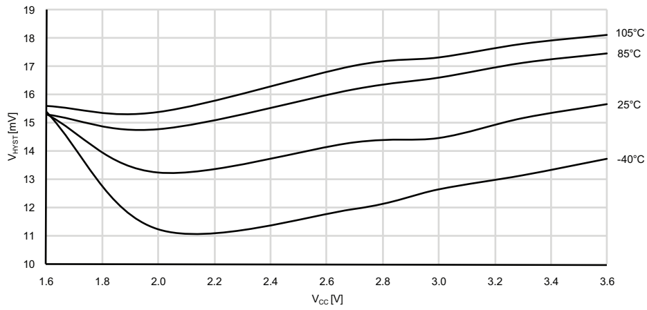
Figure 33-323. Analog Comparator Hysteresis vs. V_{CC} Small hysteresis
