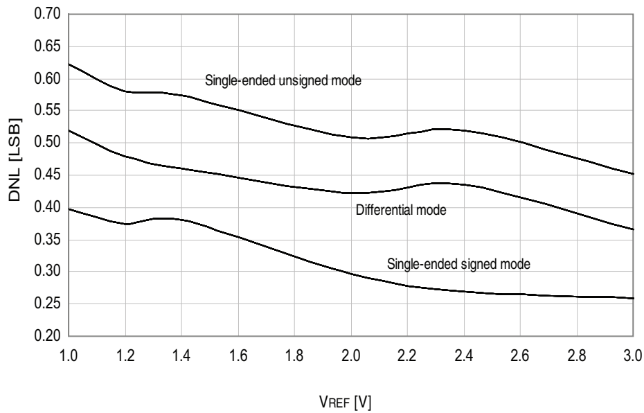
Figure 33-105. DNL Error vs. External V_{REF}
