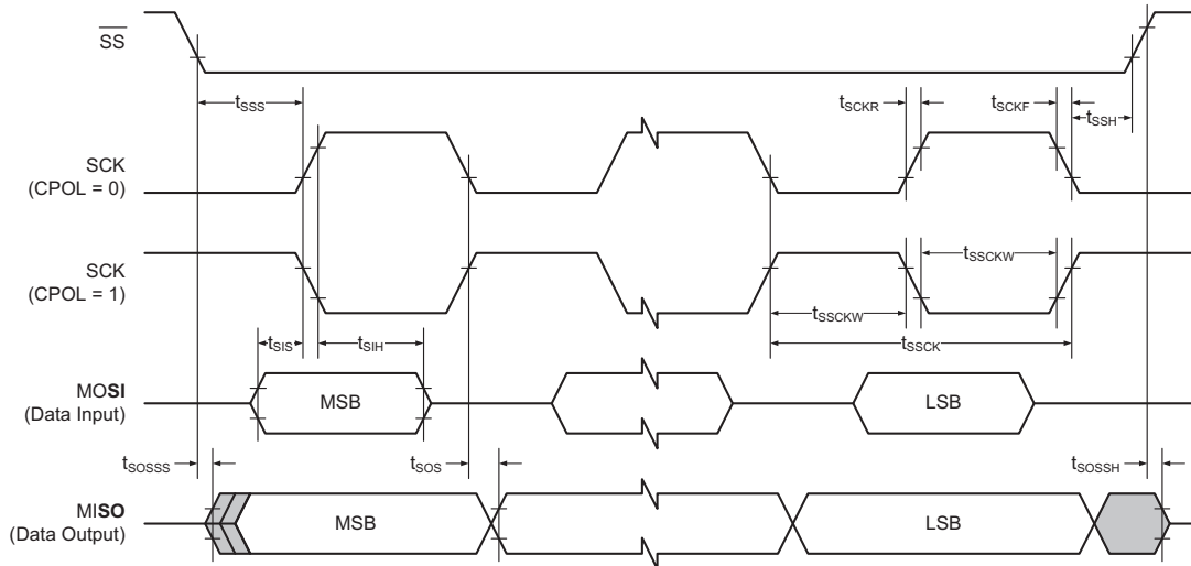
Figure 32-41. SPI Timing Requirements in Slave Mode
