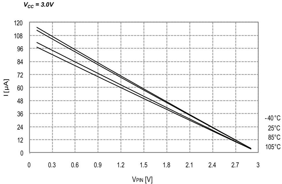
Figure 33-20. I/O Pin Pull-up Resistor Current vs. Input Voltage
