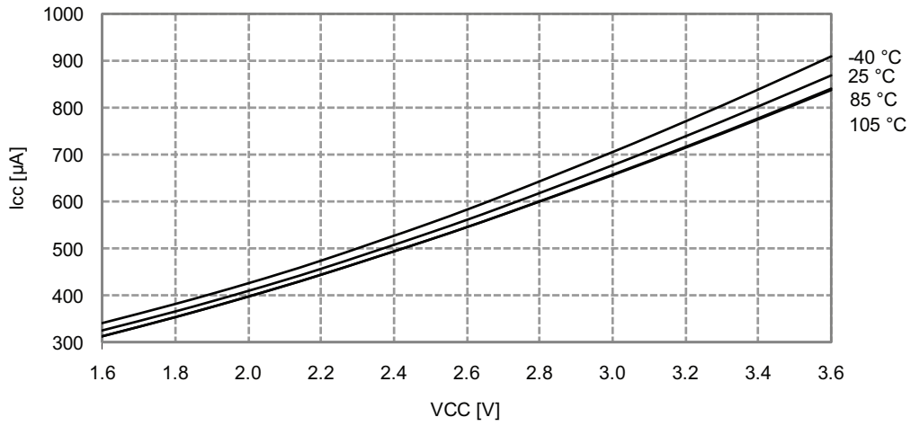
Figure 33-295. Idle Mode Supply Current vs. V CC f SYS = 32MHz internal oscillator prescaled to 8MHz
