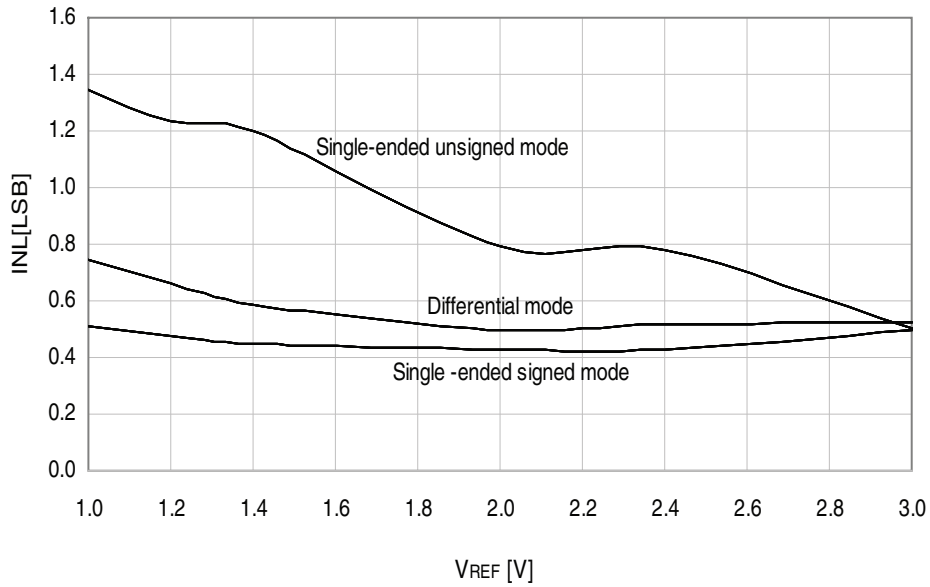
Figure 33-172. INL Error vs. External V_{REF}
