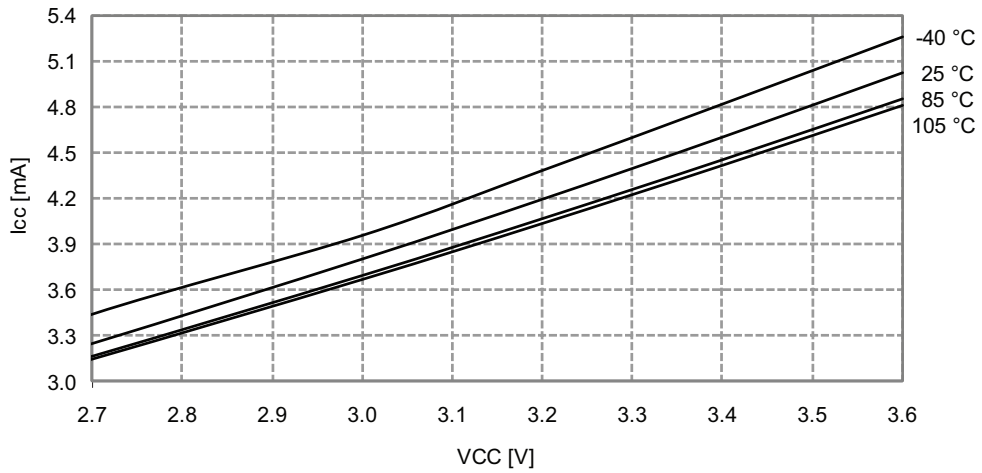
Figure 33-296. Idle Mode Current vs. V CC f SYS = 32MHz internal oscillator
