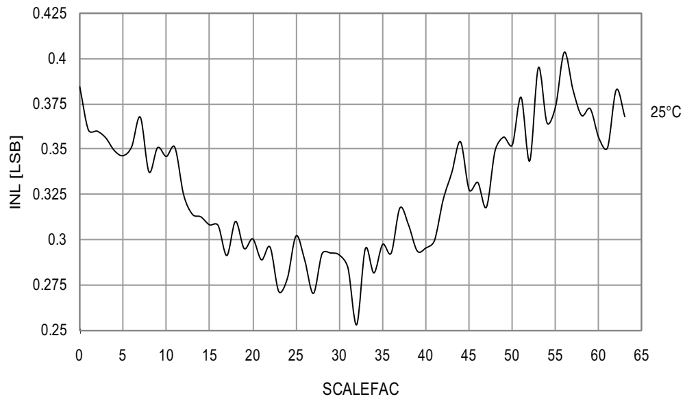
Figure 33-116. Voltage Scaler INL vs. SCALEFAC
