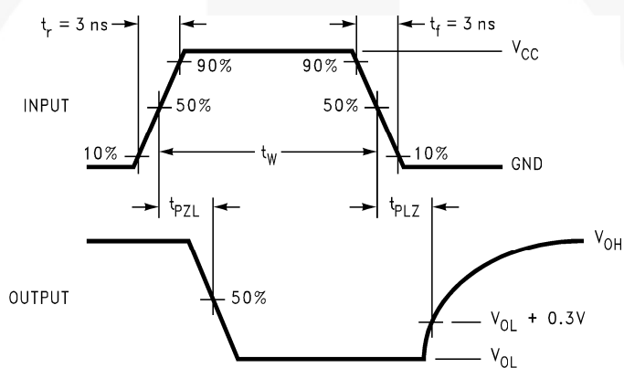
Figure 10. AC Waveforms
