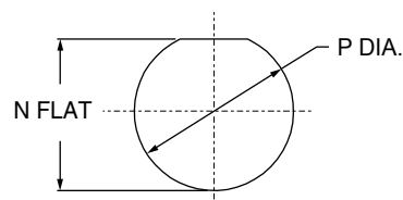
PANEL CUTOUT
