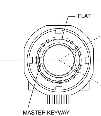
8-13 MASTER KEYWAY LOCATION
