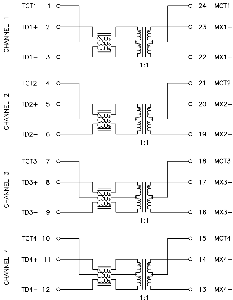
SCHMATIC
