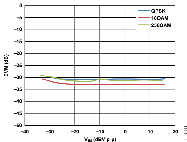
Figure 75. EVM vs. Input Voltage over Modulation Type; Filter Corner = 63 MHz, QPSK, 50 MSPS, Gain Code = 0000000, 1.5 V p-p Differential Output Level Maintained
