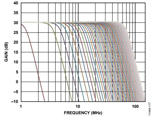
Figure 18. Gain vs. Frequency over BW Setting (Log); VGN1 = 1 V, VGN2 = 0.7 V, VGN3 = 0.75 V
