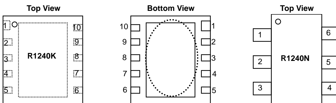
DFN(PLP)2527-10 Pin Configuration
