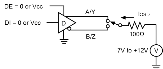
Figure 10: Driver Short Circuit Current Limit Test
