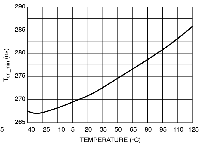
Figure 27. Minimum on Time @ R_{t\_on\_min} = 0 \Omega
