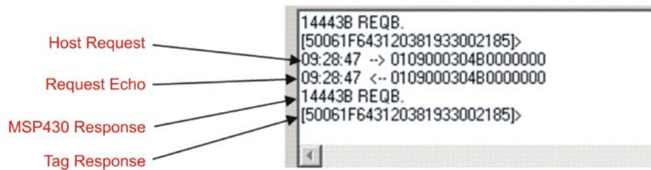
Figure 4-7: Log Window
