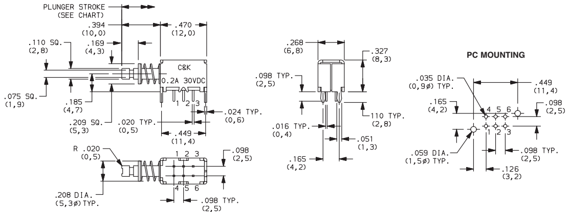
PN21SBSA03QE DPDT
