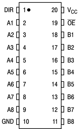
Figure 2. PIN ASSIGNMENT
