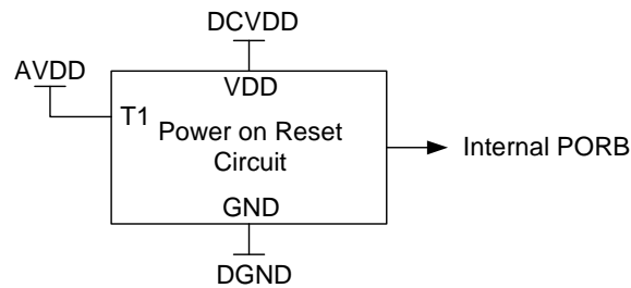
Figure 6 Internal Power on Reset Circuit Schematic
