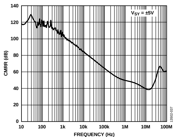
Figure 36. CMRR vs. Frequency, V_{SV} = \pm 5\text{ V}
