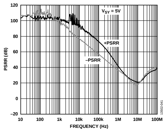
Figure 40. PSRR vs. Frequency, V_{SV} = 5\text{ V}
