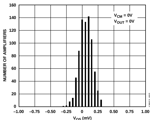
Figure 5. Input Offset Voltage ( V_{OS} ) Distribution, V_{SY} = \pm 15\text{ V}
