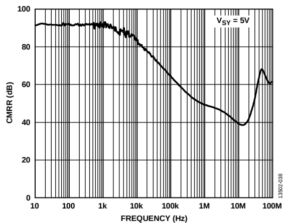
Figure 37. CMRR vs. Frequency, V_{SV} = 5\text{ V}
