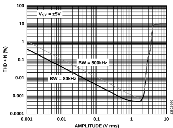
Figure 69. THD + Noise vs. Amplitude, V_{SV} = \pm 5 V
