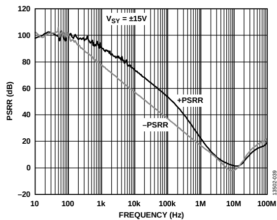
Figure 38. PSRR vs. Frequency, V_{SV} = \pm 15\text{ V}
