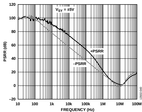
Figure 39. PSRR vs. Frequency, V_{SV} = \pm 5\text{ V}
