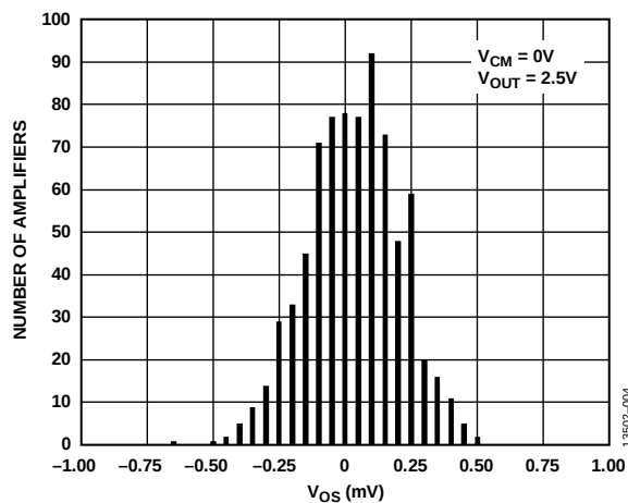
Figure 7. Input Offset Voltage ( V_{OS} ) Distribution, V_{SY} = 5\text{ V}
