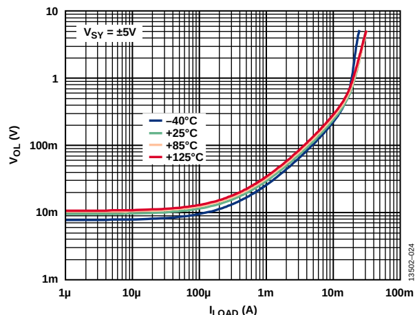
Figure 23. Output Voltage High ( V_{OH} ) to Supply Rail vs. Load Current ( I_{LOAD} ) over Temperature, V_{SY} = \pm 5 V
