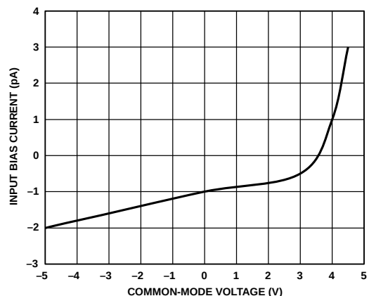
Figure 77. Input Bias Current vs. Common-Mode Voltage with \pm 5\text{ V} Supply
