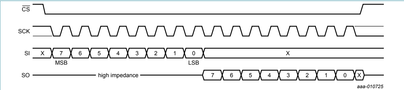
Figure 3. SPI mode 0/3
