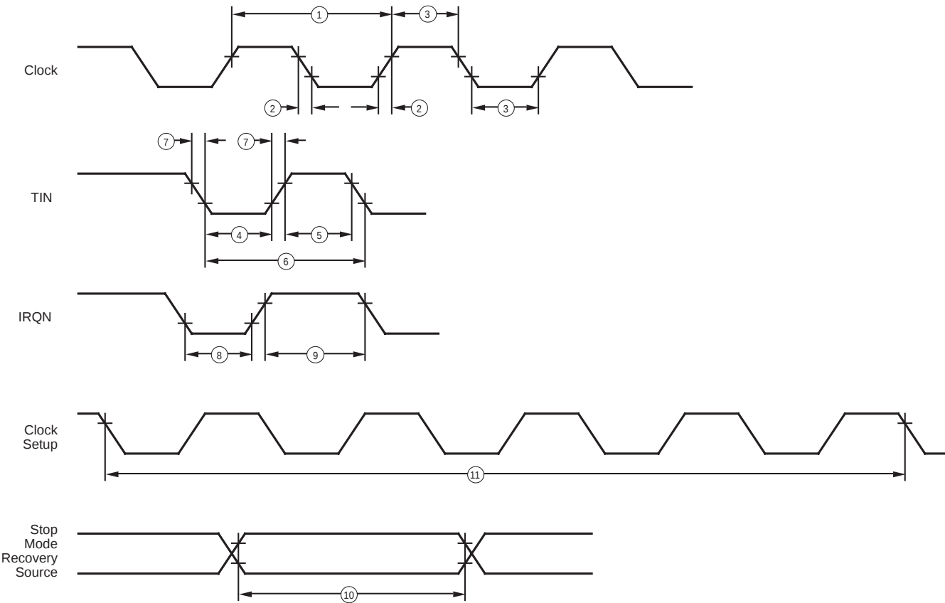
Figure 4. Additional Timing
