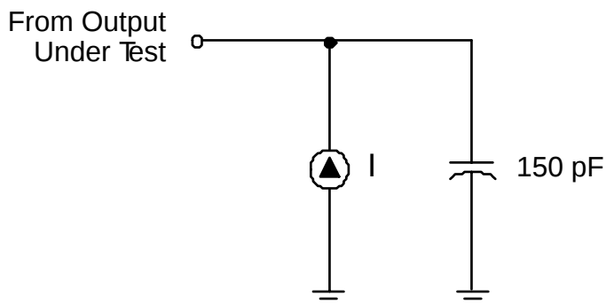
Figure 3. Test Load Diagram
