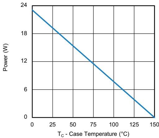
Power, Junction-to-Case
