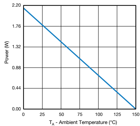
Power, Junction-to-Ambient
