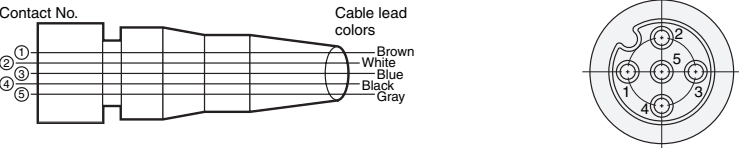
Wiring Diagram
