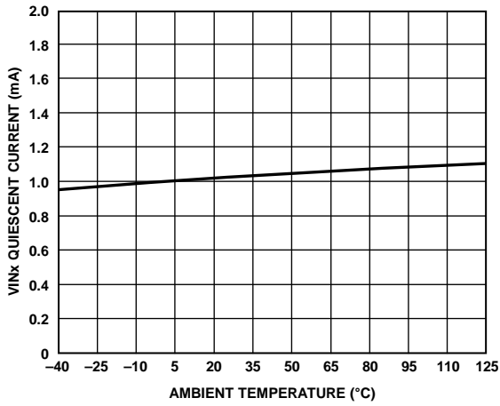
Figure 12. V_{INx} Quiescent Current vs. Ambient Temperature, DIS\_LDO = High
