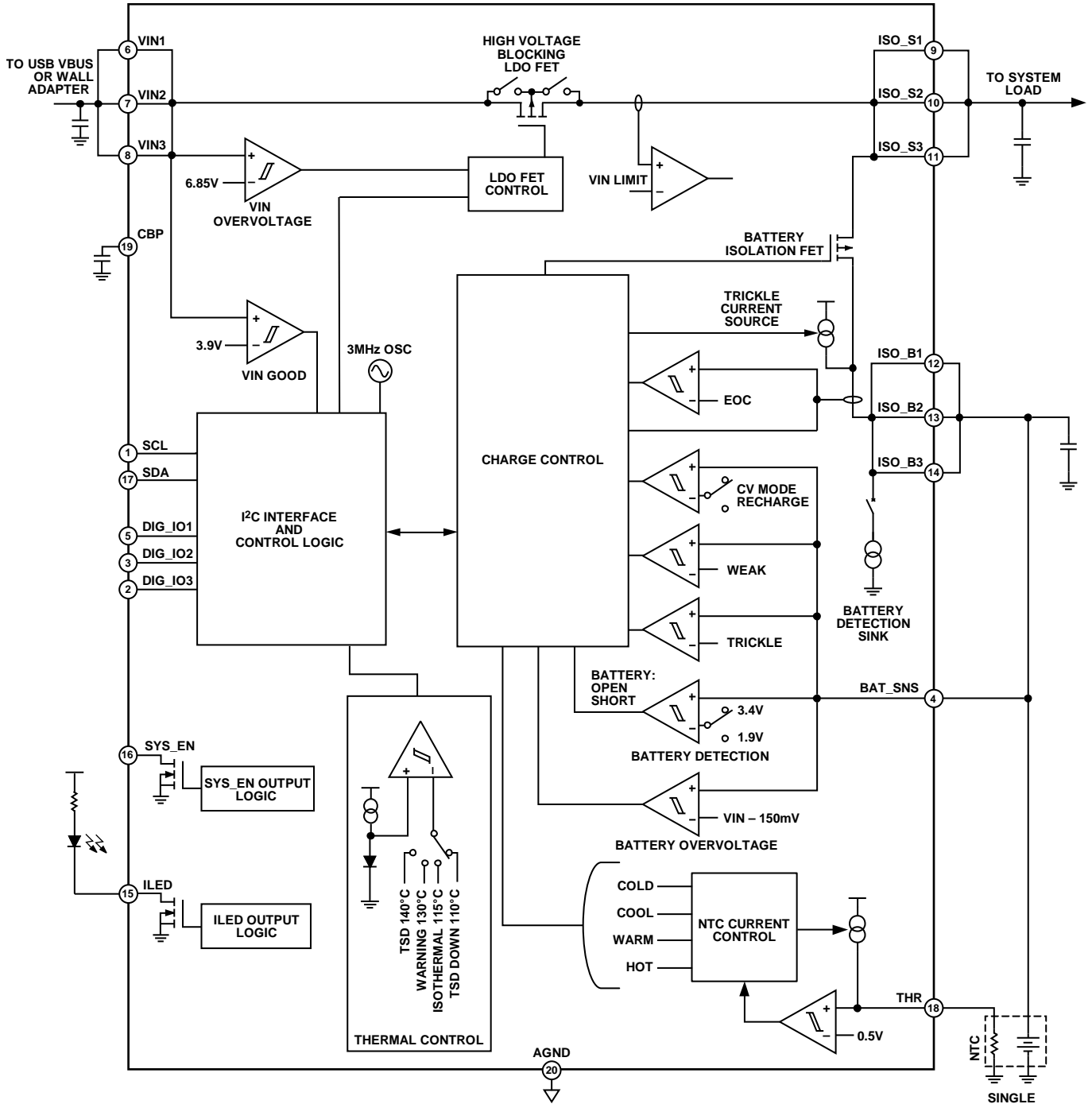
Figure 26. Block Diagram
