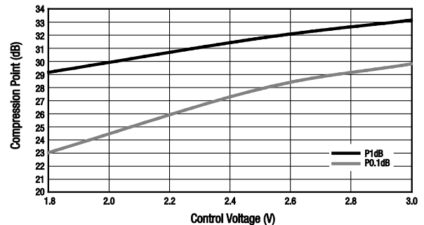
Figure 8. P1dB and PO.1dB vs Control Voltage @ 5.5 GHz
