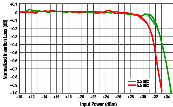
Figure 7. Insertion Loss vs Input Power @ 2.5 GHz and 5.5 GHz
