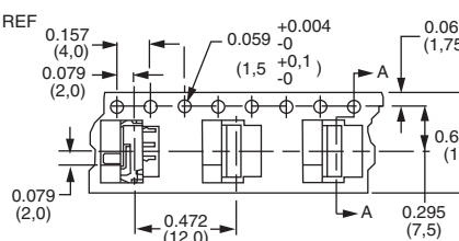
CARRIER TAPE
