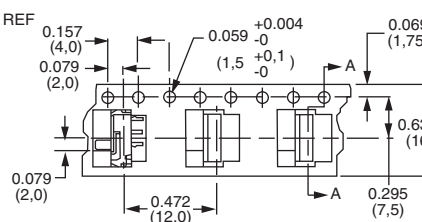
CARRIER TAPE
