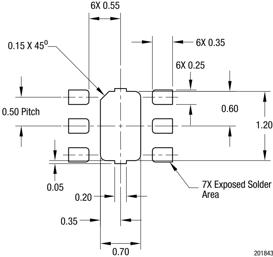
Figure 10. SKY13446-374LF PCB Layout Footprint (Top View)
