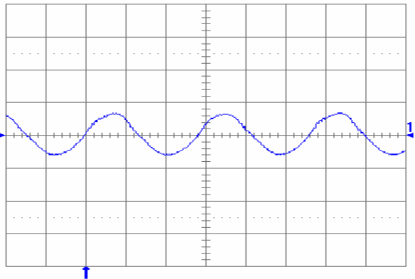
Fig. 11: Output voltage ripple (50 mV/div.) at full rated load current into a resistive load with C_o = 10\ \mu\text{F} tantalum + 1 \mu\text{F} ceramic and V_{in} = 48\text{ V} . Time scale: 1 \mu\text{s} /div.
