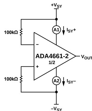
Figure 75. Comparator A
