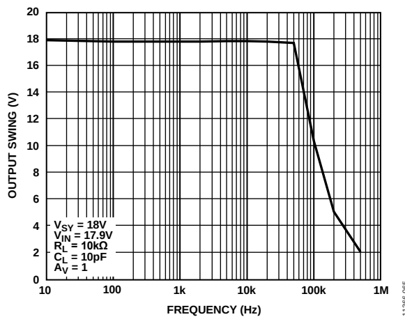
Figure 64. Output Swing vs. Frequency
