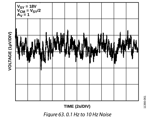
Figure 63. 0.1 Hz to 10 Hz Noise
