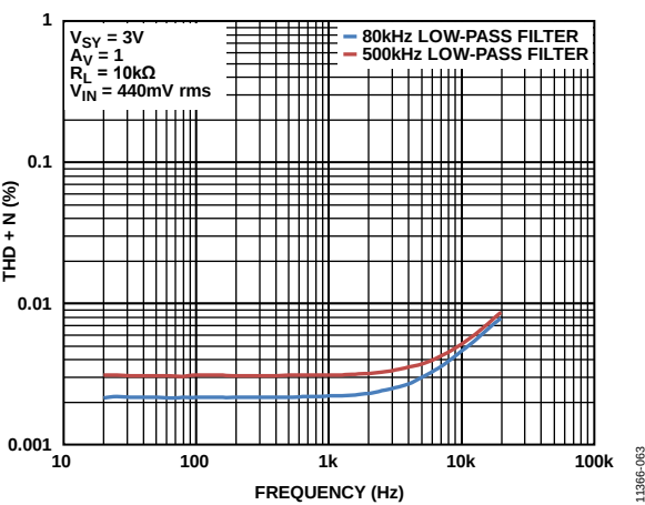
Figure 62. THD + N vs. Frequency
