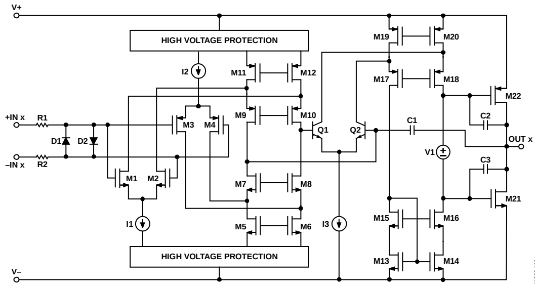
Figure 70. Simplified Schematic
