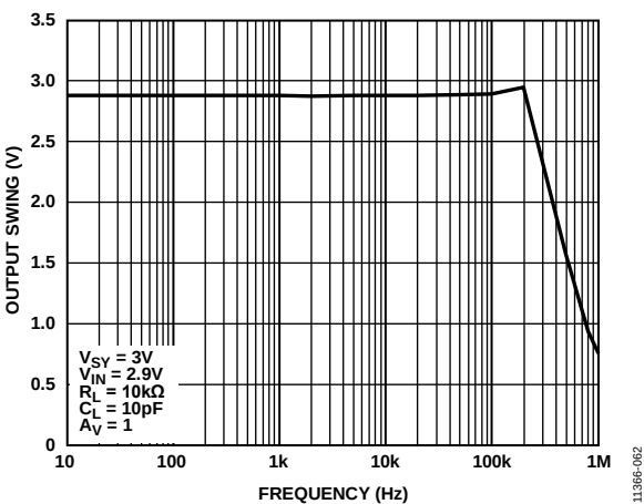
Figure 61. Output Swing vs. Frequency
