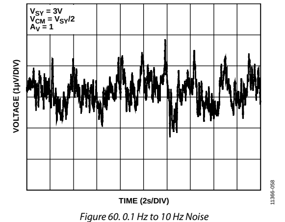
Figure 60. 0.1 Hz to 10 Hz Noise
