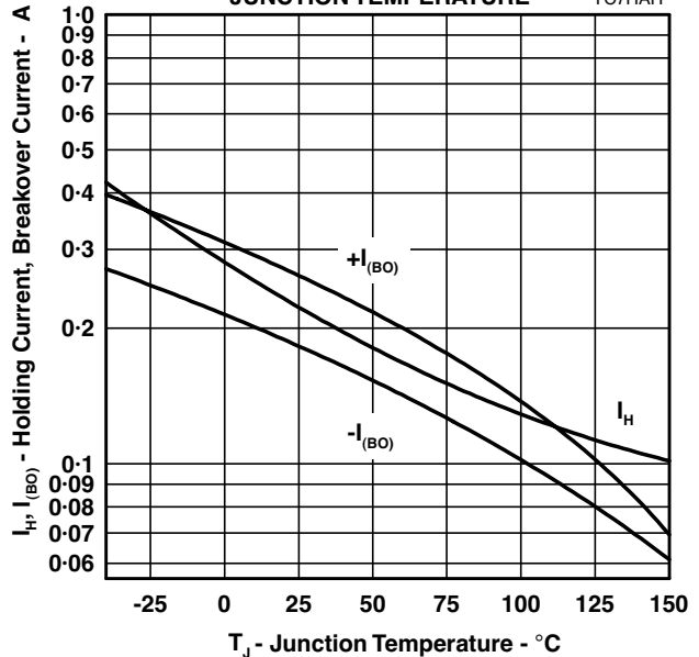
HOLDING CURRENT & BREAKOVER CURRENT vs JUNCTION TEMPERATURE
