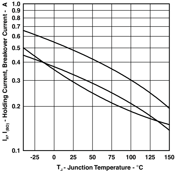
HOLDING CURRENT & BREAKOVER CURRENT
