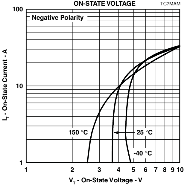
TISP7125F3 THRU TISP7180F3 ON-STATE CURRENT vs ON-STATE VOLTAGE
