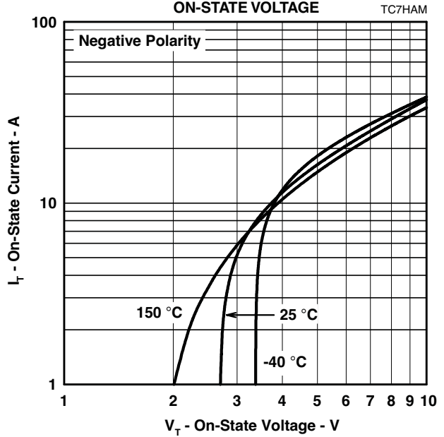
TISP7240F3 THRU TISP7380F3 ON-STATE CURRENT vs ON-STATE VOLTAGE
