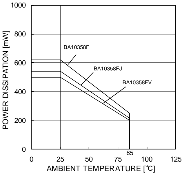
Figure 2. Derating Curve
