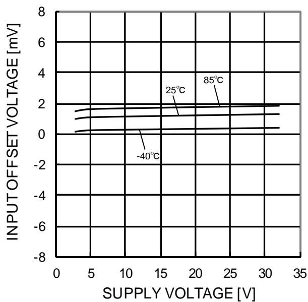
Figure 37. Input Offset Voltage - Supply Voltage (VICM=0V, OUT=1.4V)
