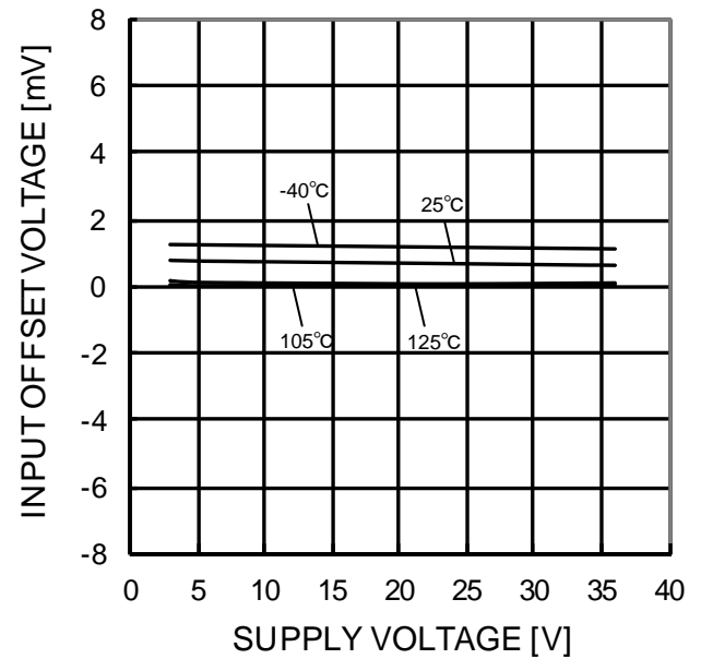
Figure 85. Input Offset Voltage - Supply Voltage (VICM=0V, OUT=1.4V)
