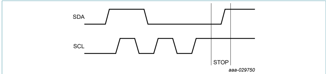
Figure 18. I 2 C stop condition
