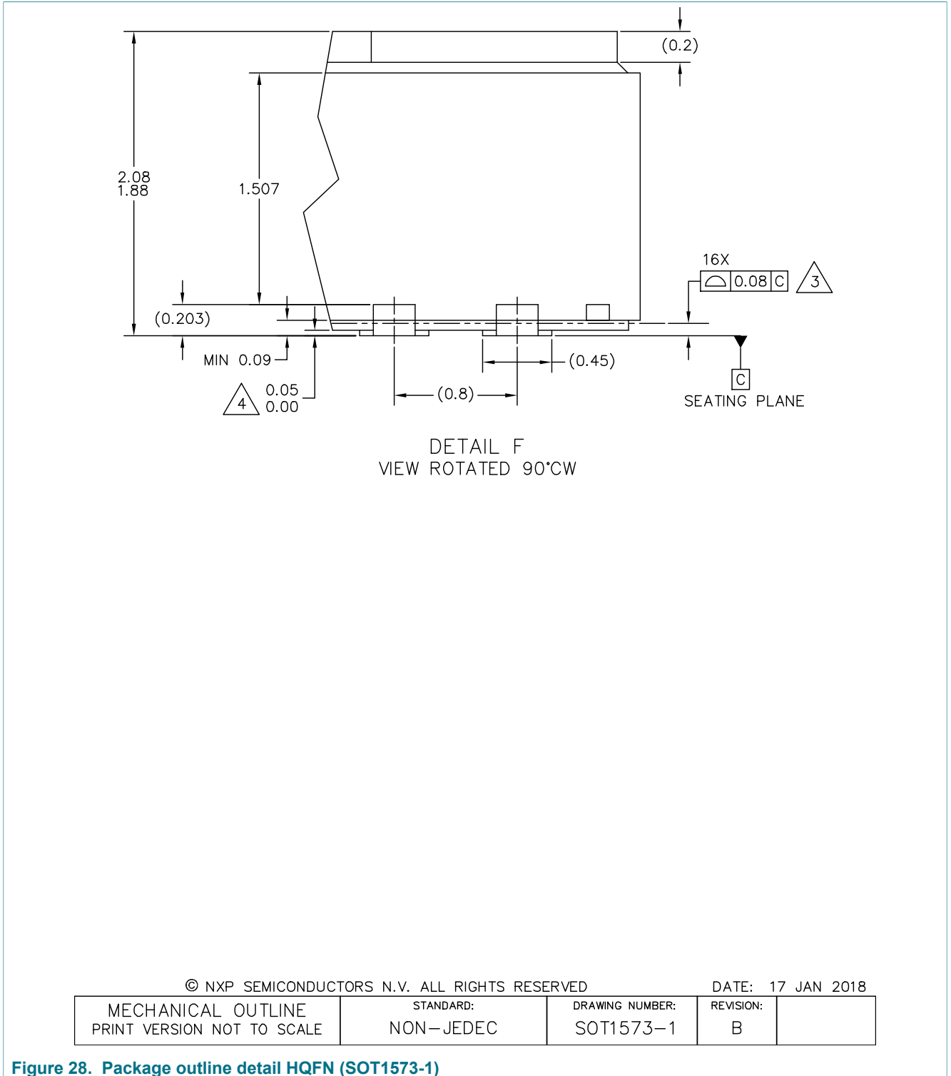
Figure 28. Package outline detail HQFN (SOT1573-1)
