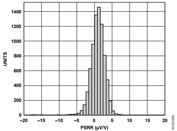
Figure 6. Typical Distribution of PSRR (G = 1)
